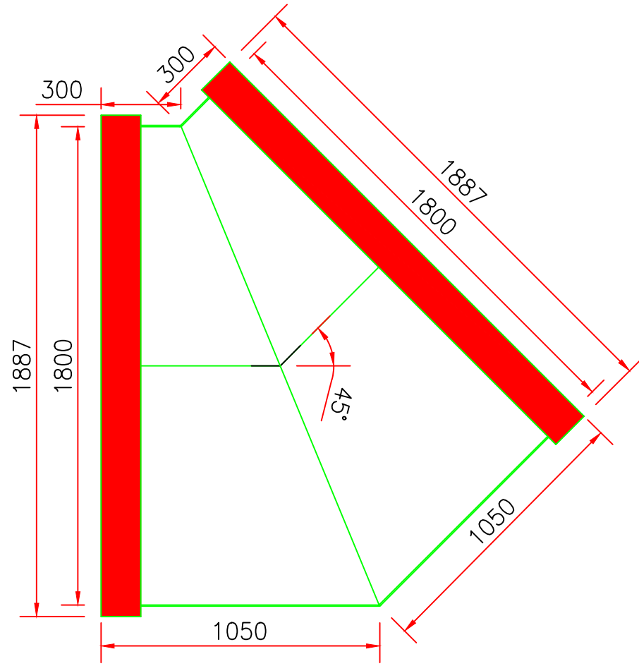
1800 \phi STAINLESS STEEL 45° BEND (SCALE 1/20)
